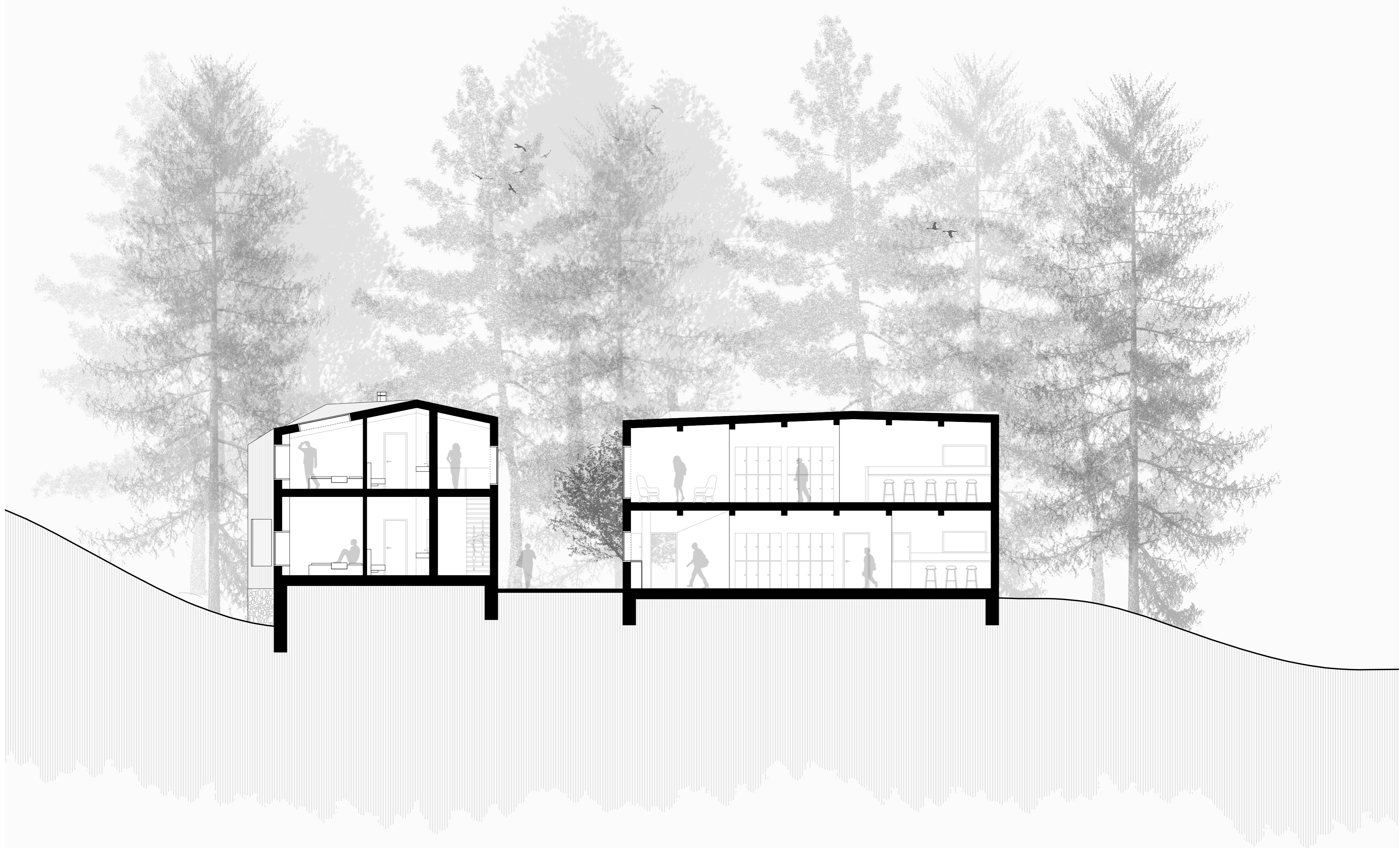
HOUSING ANSICHT WEST M 1:100
