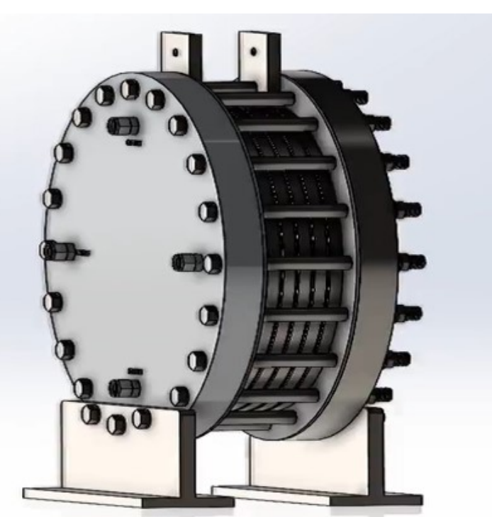
COMSOL: Stack Model (Numerical)
