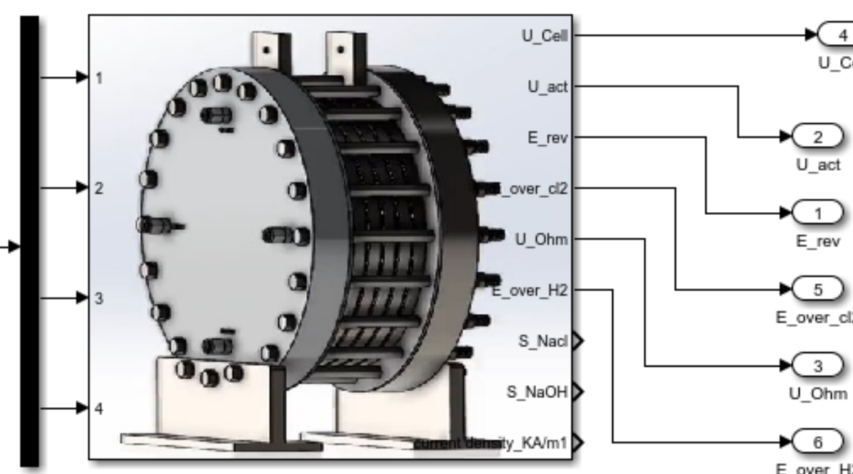
MATLAB/Simulink: Stack Model
