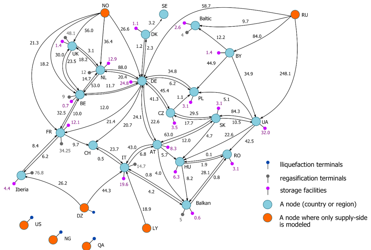
Figure 2: Nodes included in the model and capacities of gas infrastructure elements for 2017 (in bcm p.a.). 13
